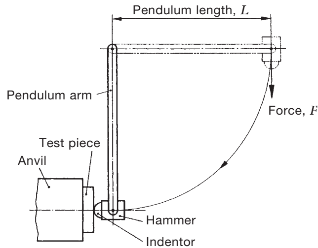
Figure 1: Principle of test apparatus
